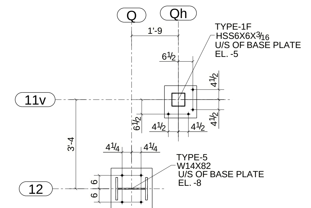
DETAIL A
