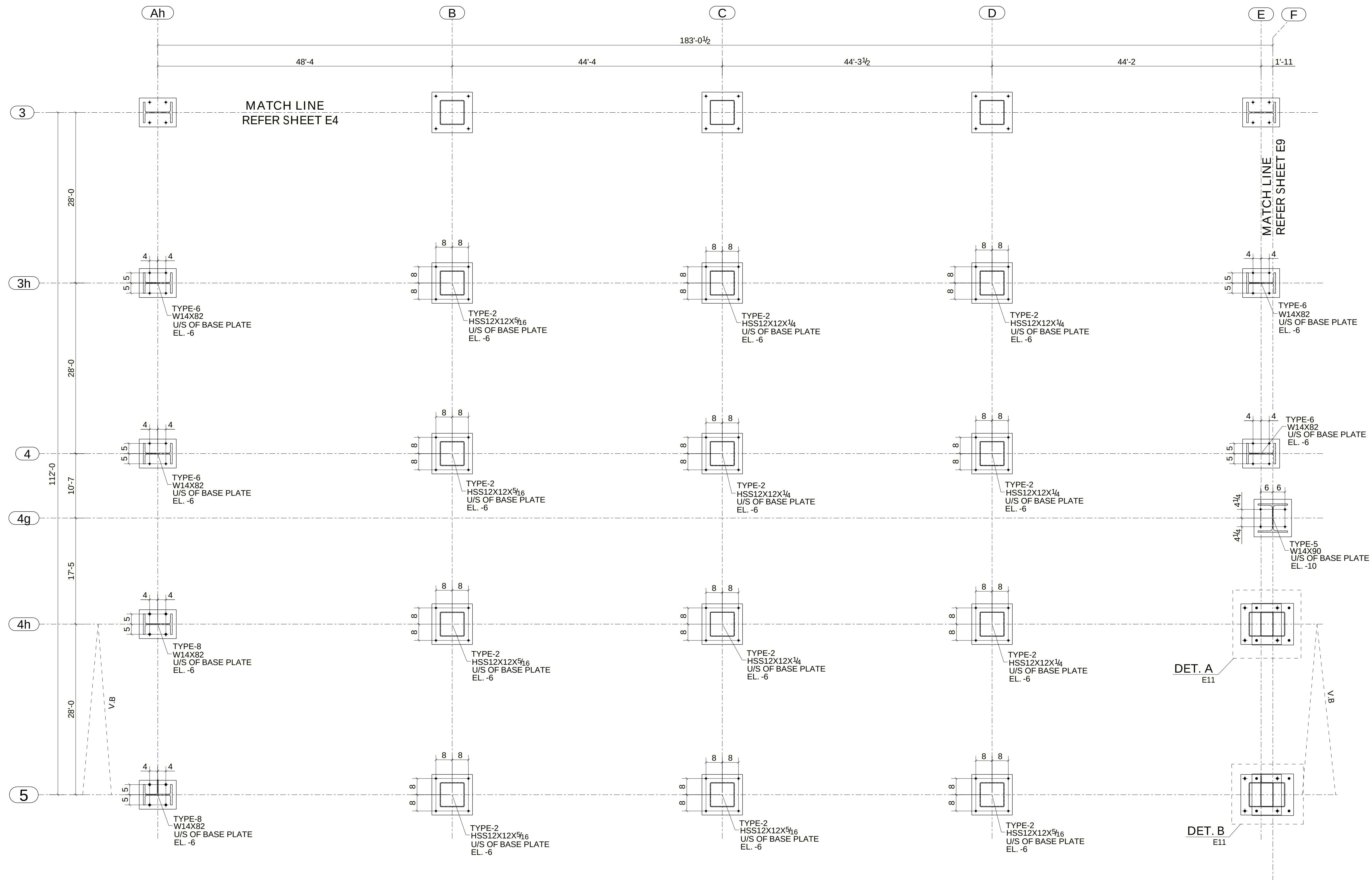
PARTIAL ANCHOR BOLT PLAN (REFER SHEET:S201)
