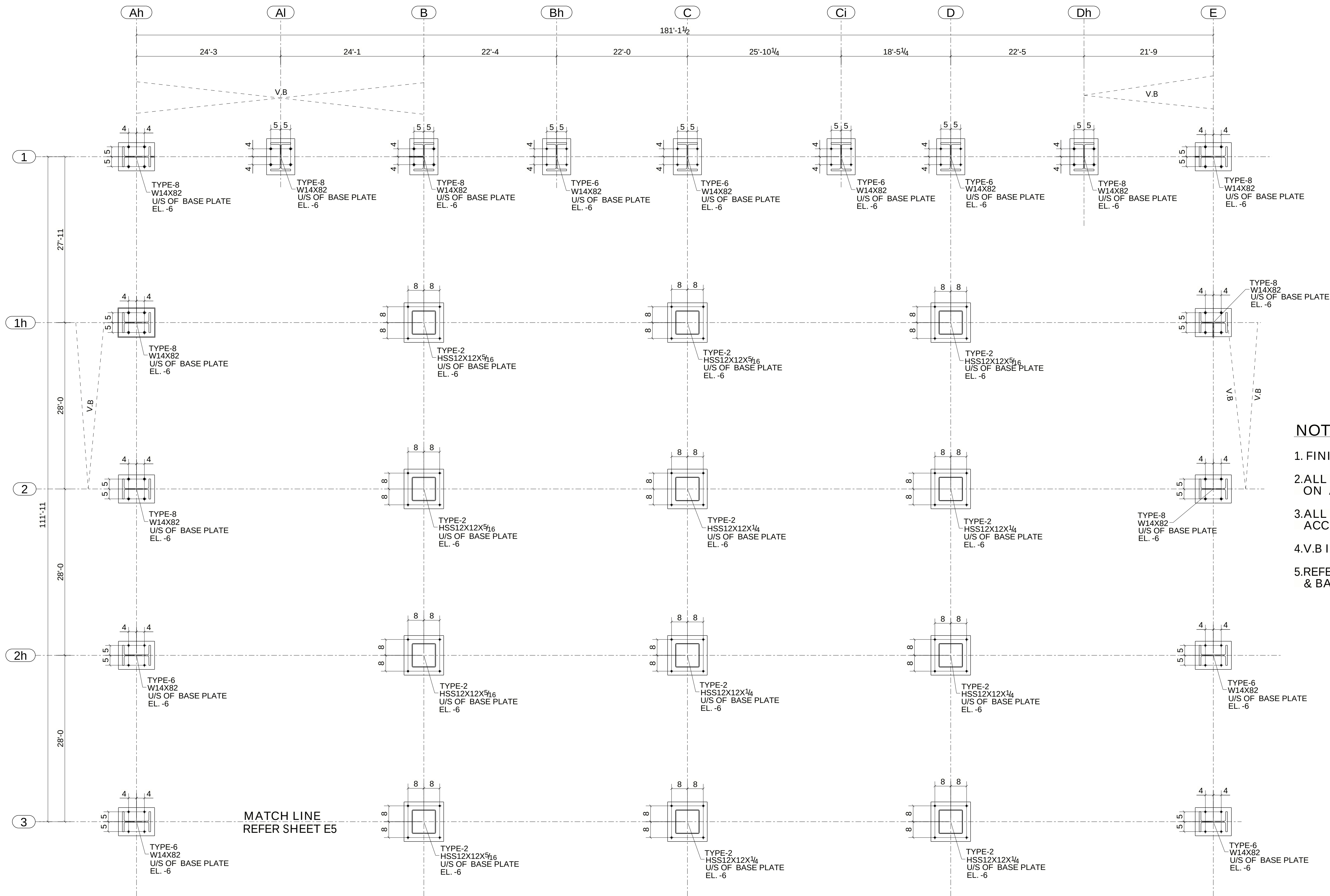
PARTIAL ANCHOR BOLT PLAN (REFER SHEET:S201)
