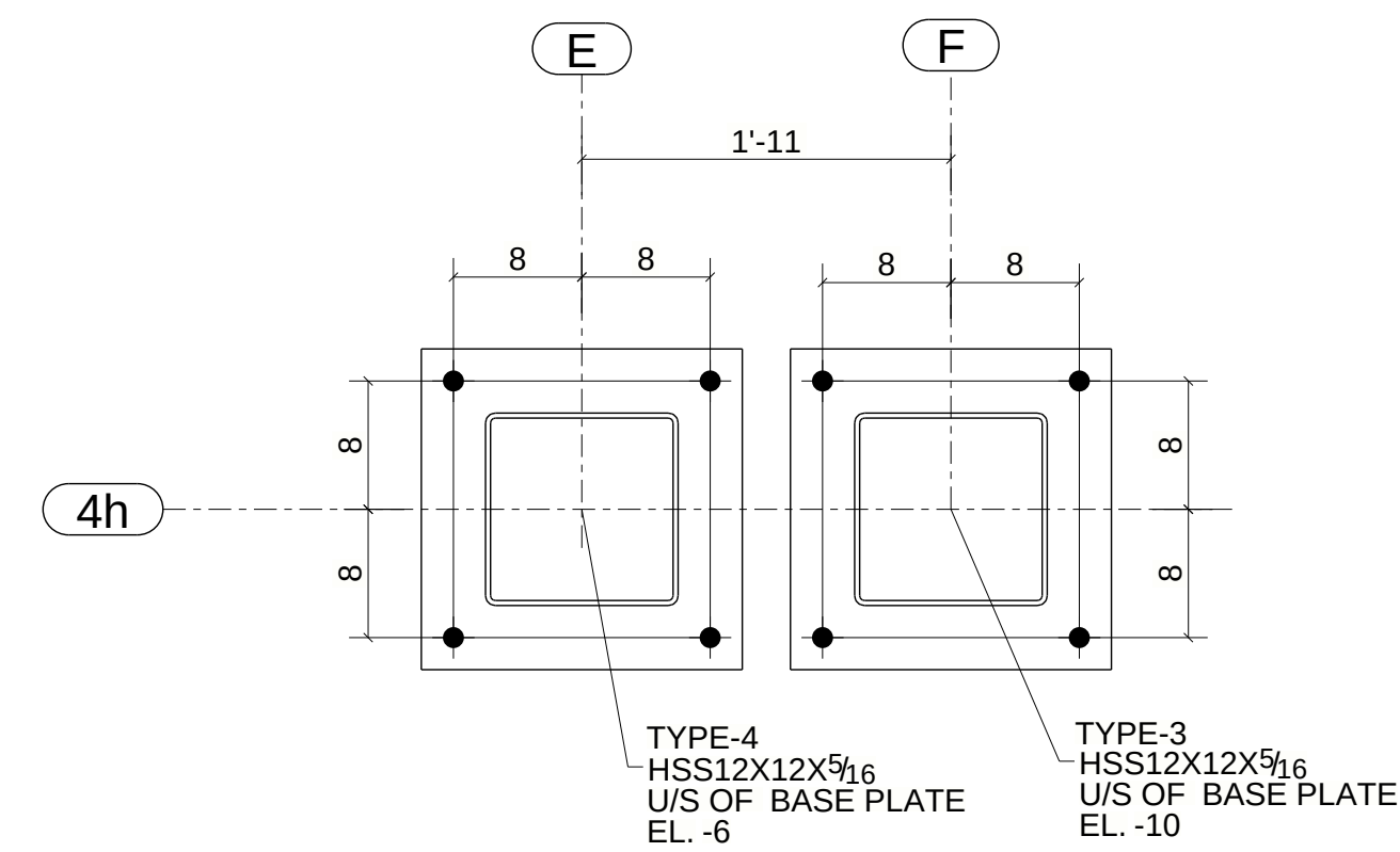
DETAIL A E5
