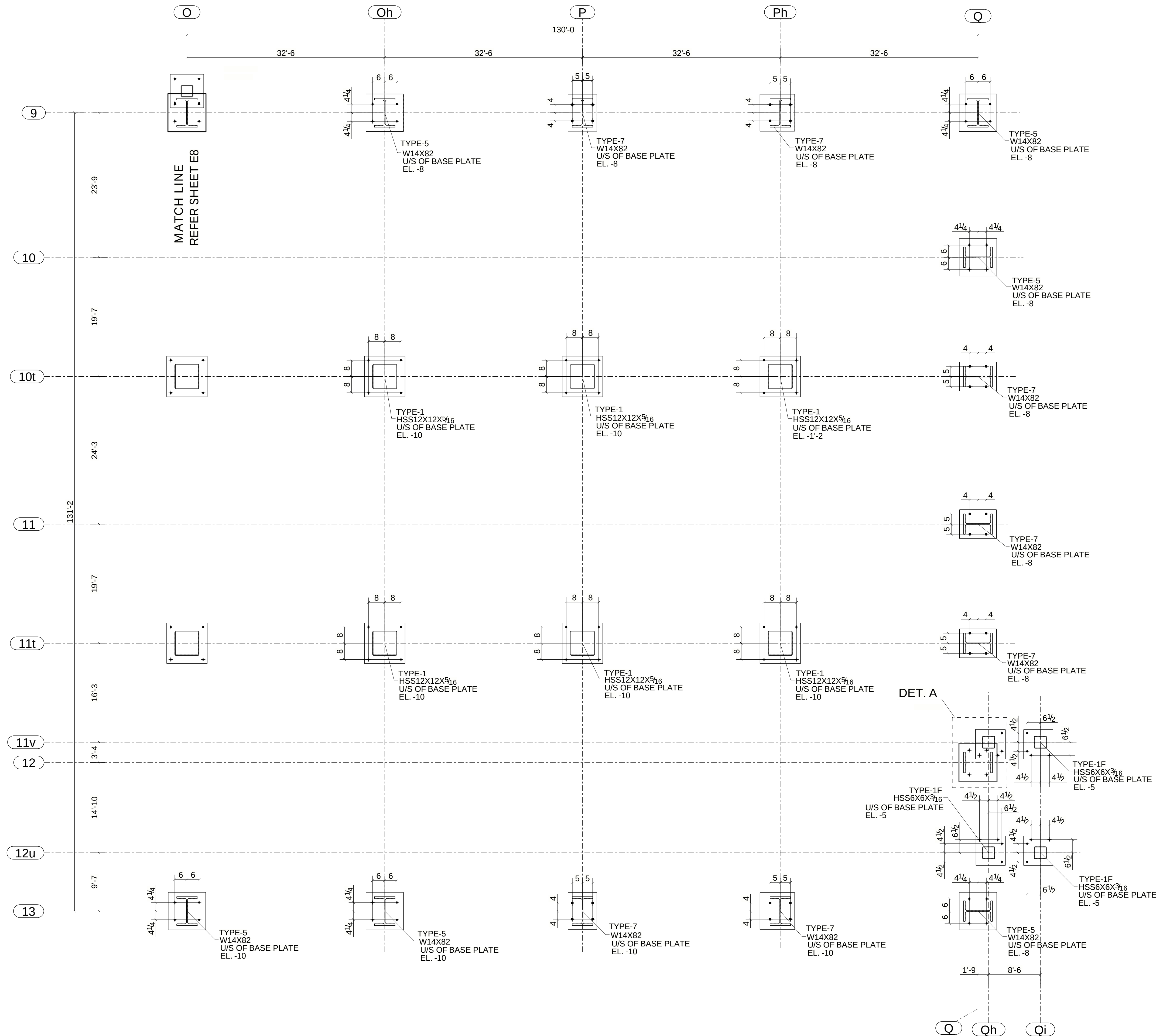
PARTIAL ANCHOR BOLT PLAN REFER SHEET: S202
