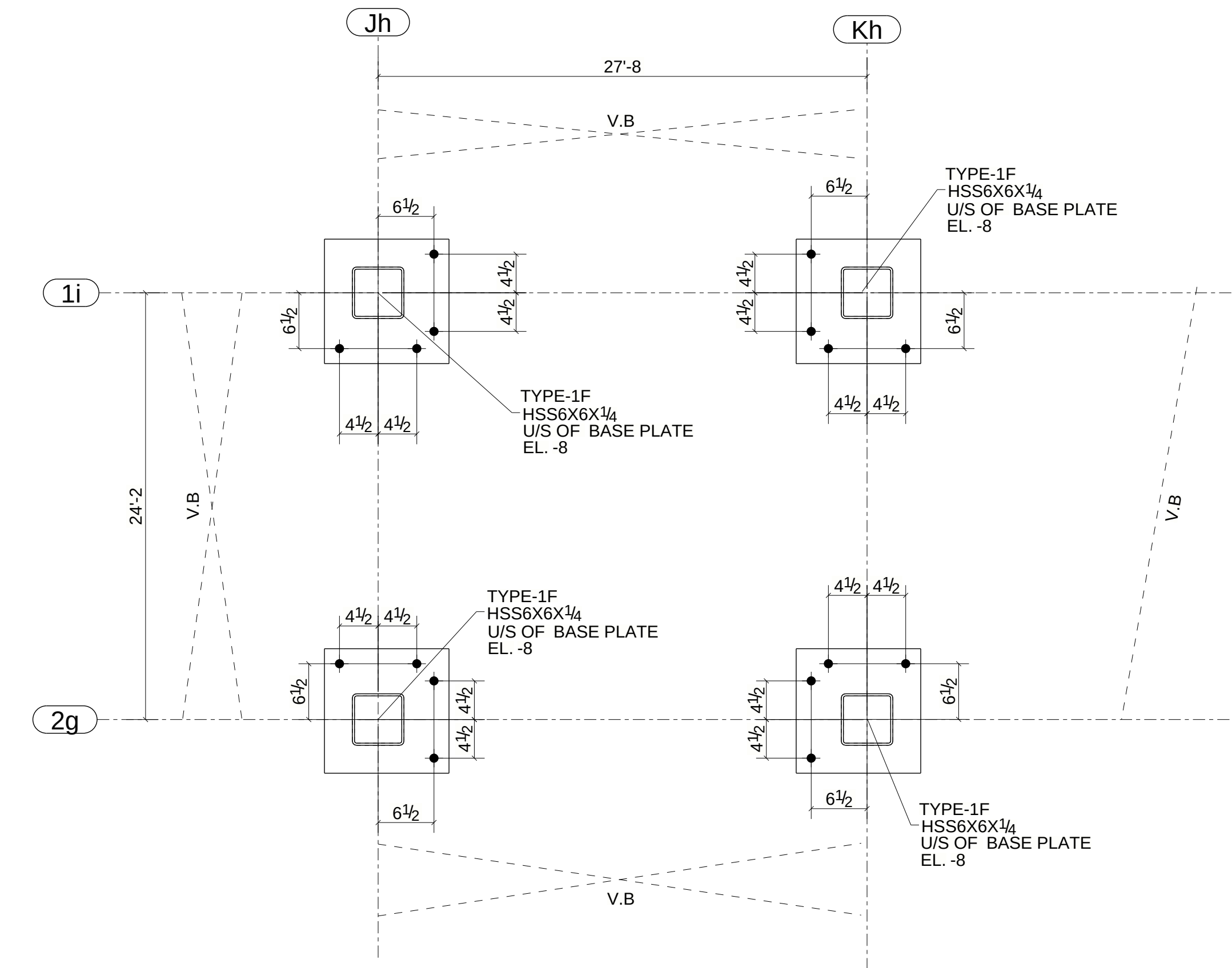
PARTIAL ANCHOR BOLT PLAN@PUMP ROOM (REFER SHEET:2/S201)
