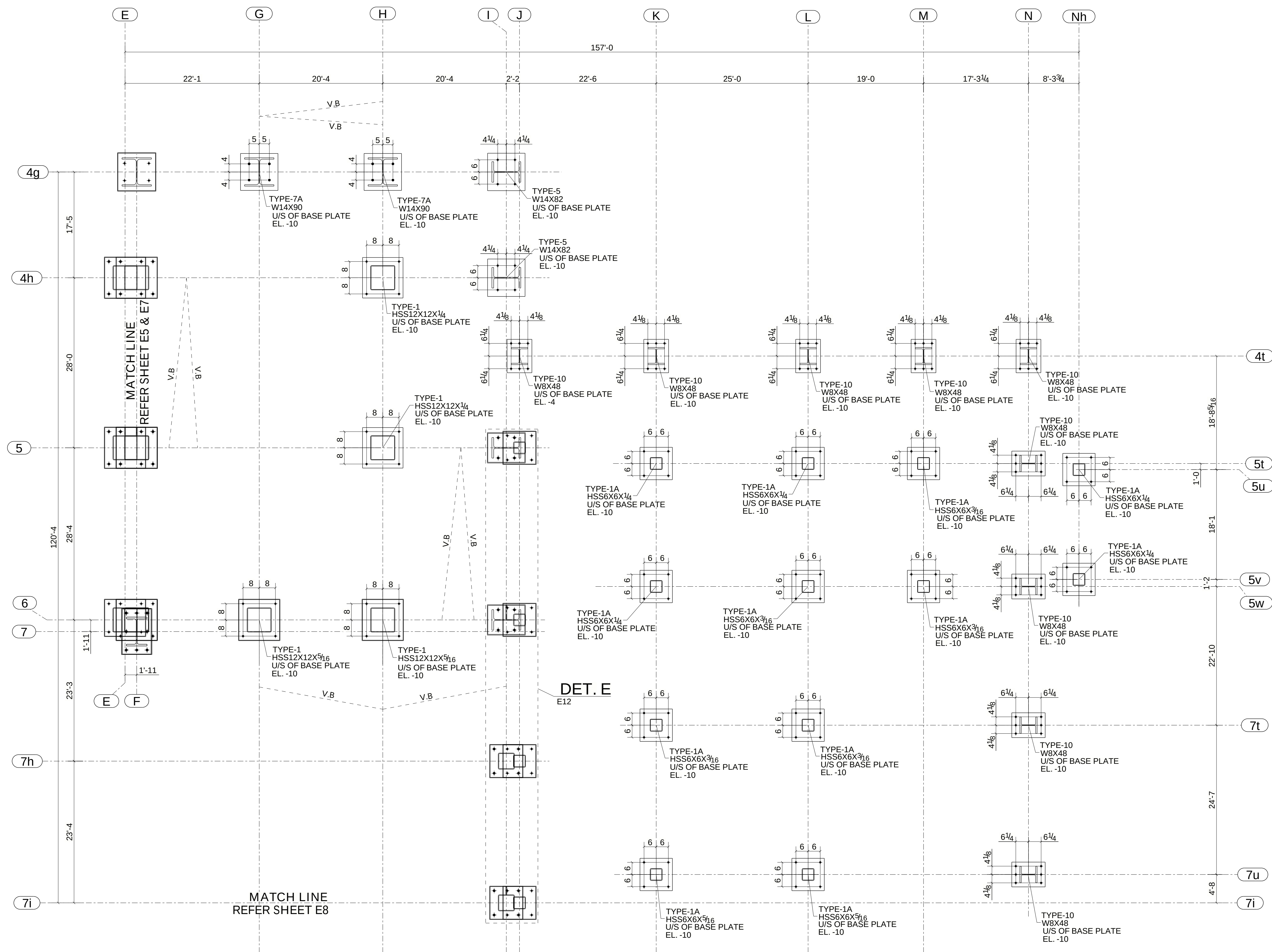
PARTIAL ANCHOR BOLT PLAN (REFER SHEET 1/S201 & 1/S203)
