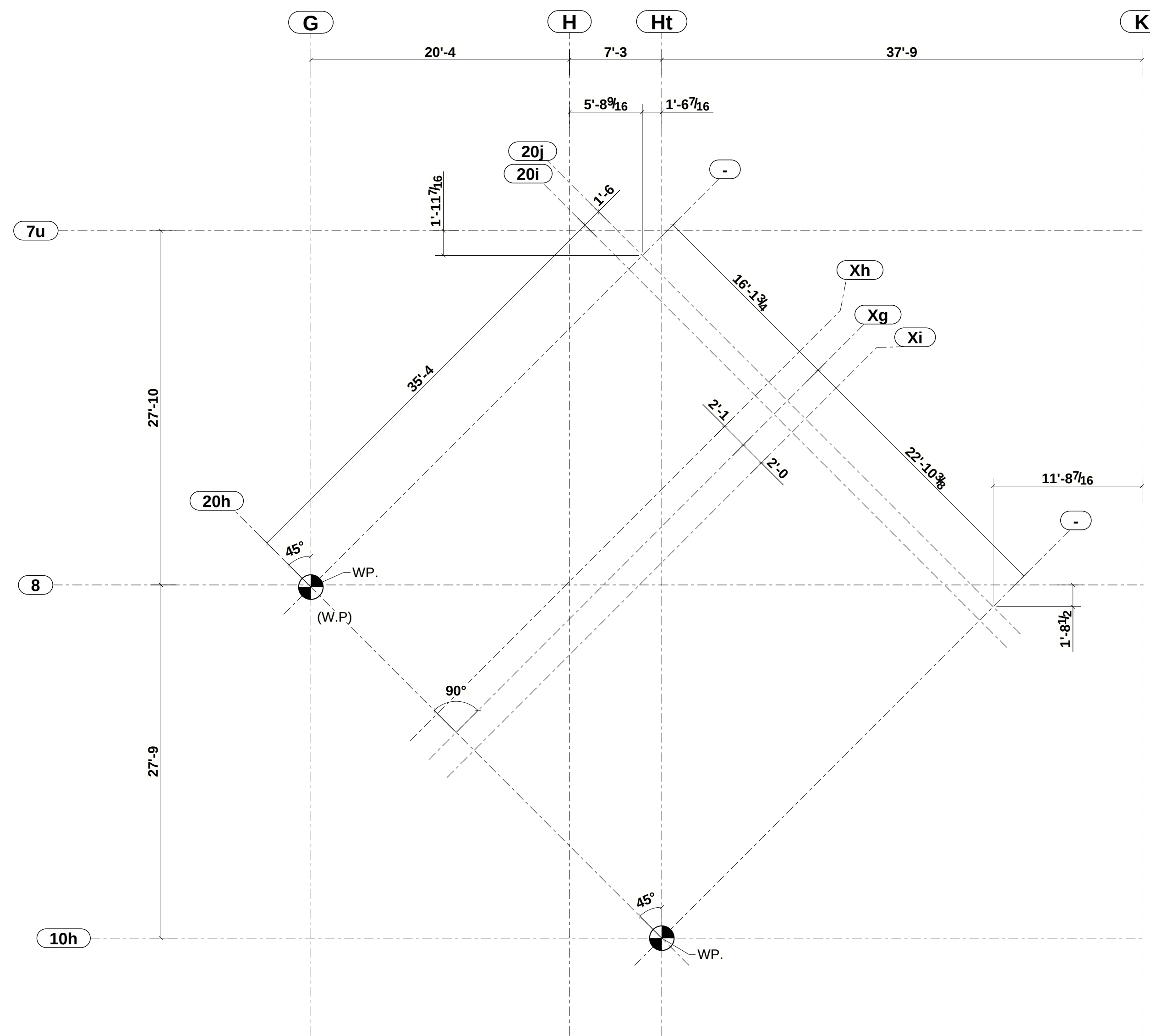
PARTIAL GRID LAYOUT
