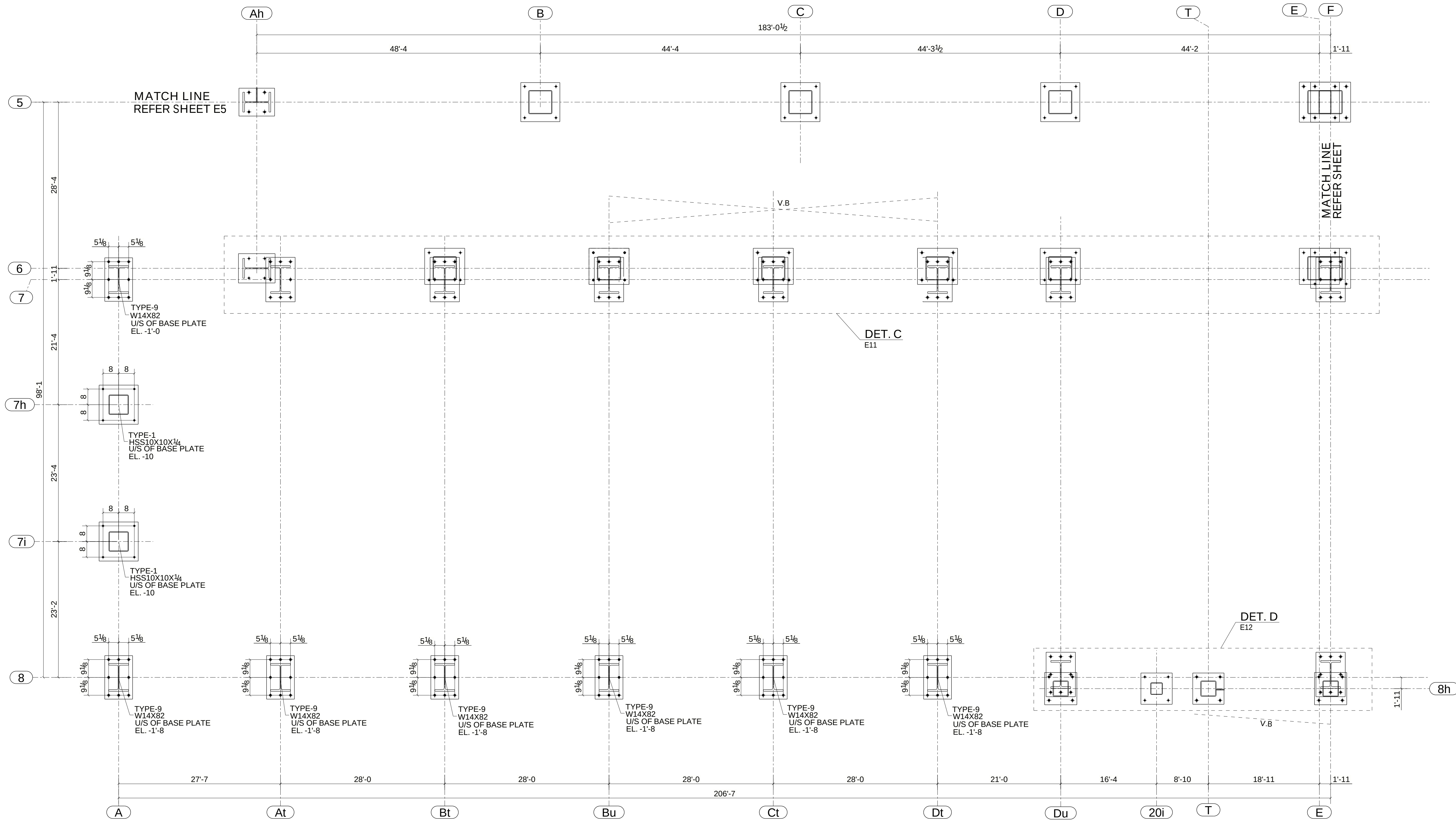
PARTIAL ANCHOR BOLT PLAN (REFER SHEET:1/S202 & 1/S201)
