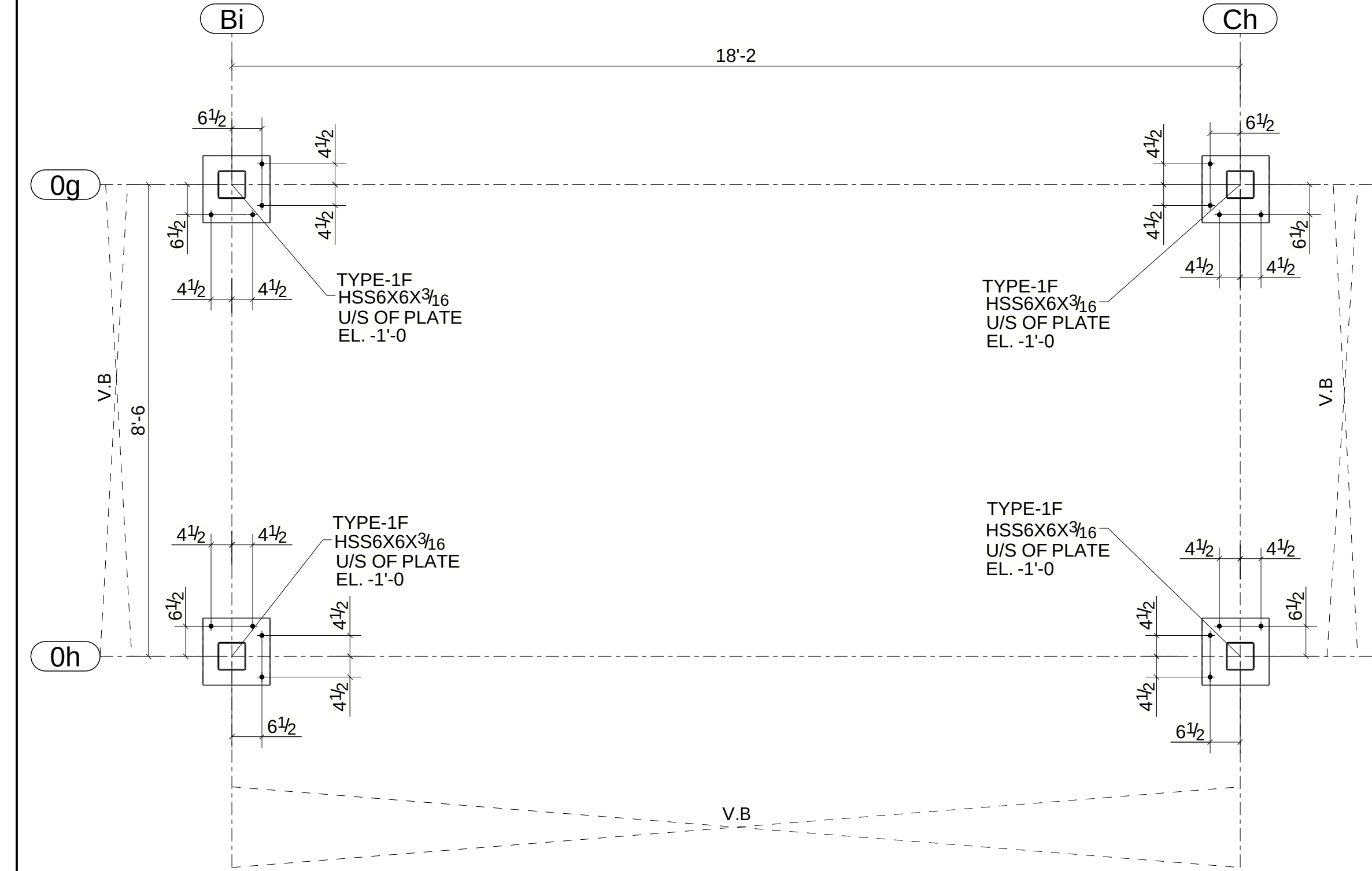
PARTIAL ANCHOR BOLT PLAN RISE ROOM FREEZER (REFER SHEET:3/S201)
