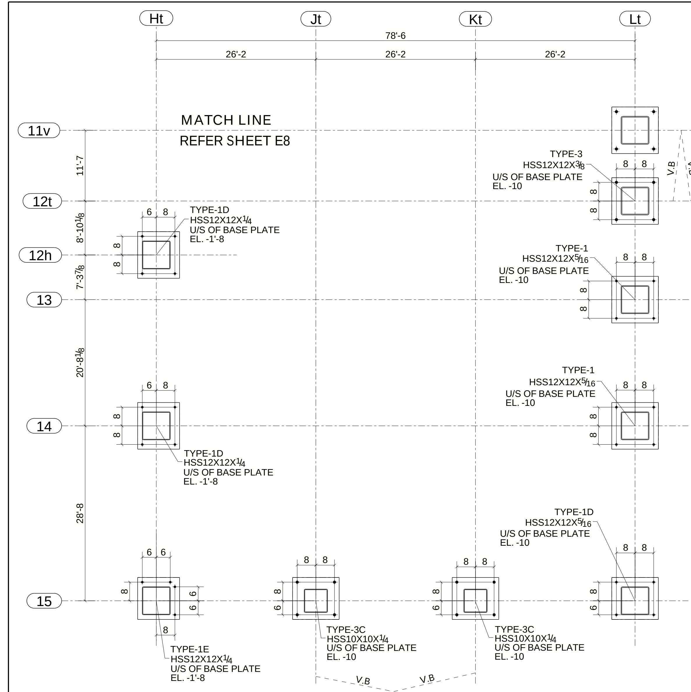
PARTIAL ANCHOR BOLT PLAN (REFER SHEET:S202)
